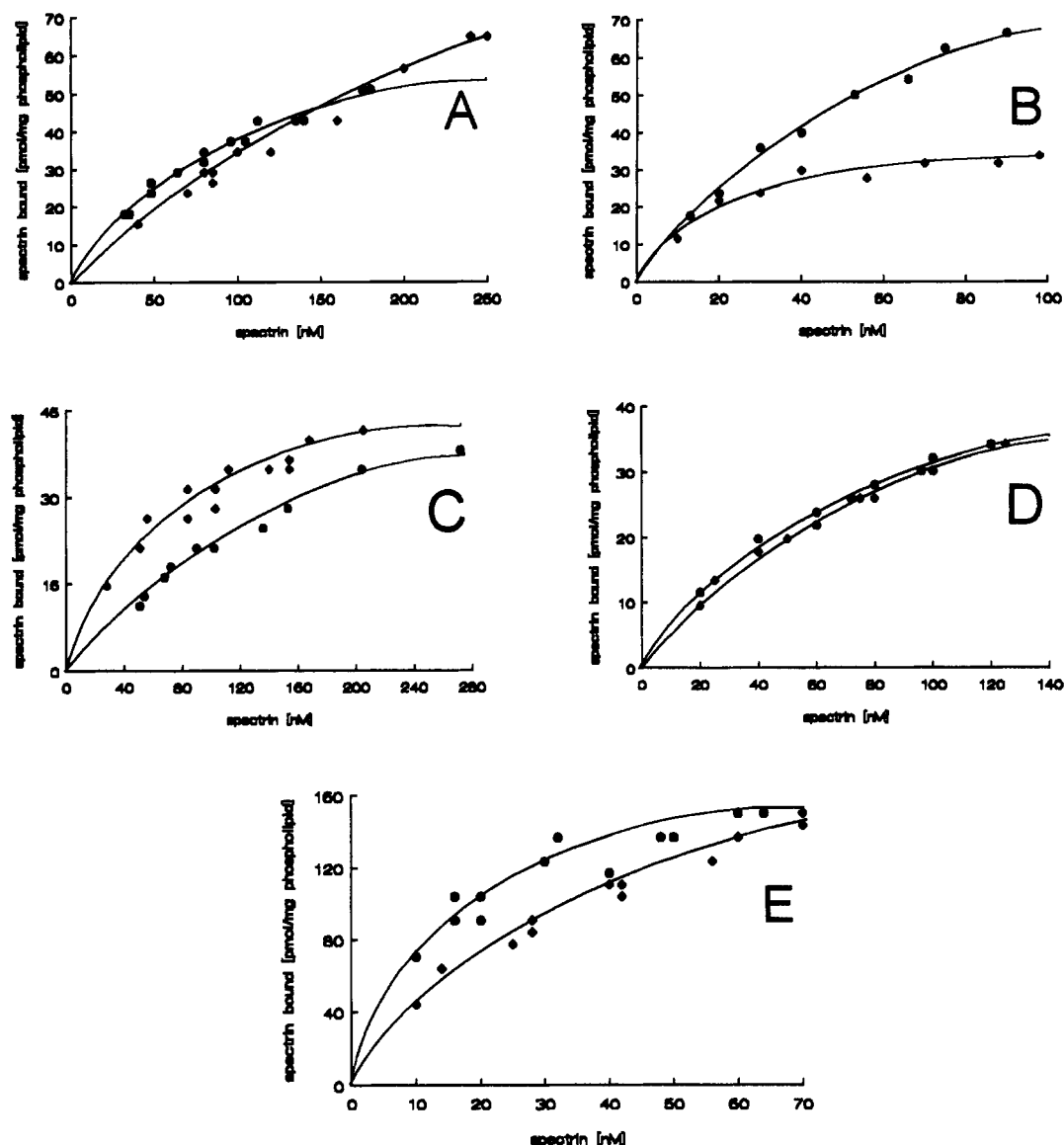
FIGURE 6: Binding of increasing concentrations of purified brain spectrin by FAT-liposomes prepared from: (A) PC, (B) PE/PC (60:40), (C) PS/PC (60:40), (D) PE/PS (60:40), and (E) total phospholipids extracted from bovine brain synaptic plasma membrane. Lipid isolation and characterization were as in the Experimental Procedures and Figure 1B. Lipid concentration (2.05 mM) was estimated as phospholipid phosphorus. Binding data obtained at pH 7.5 (●) and at pH 6.0 (◆). Other details are in the Experimental Procedures.
